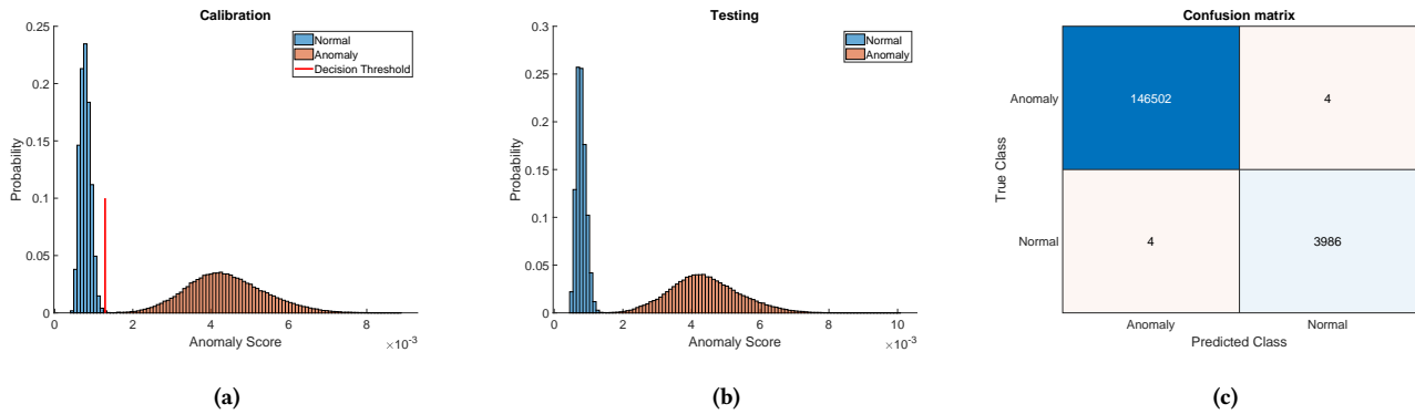
Figure 12: Outdoor moving scenario: (a) decision threshold estimation, (b) testing, and (c) confusion matrix.
