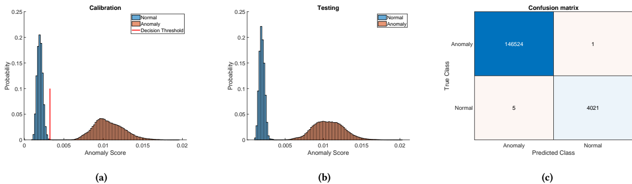
Figure 8: Outdoor scenario, static receiver with LoS: (a) decision threshold estimation, (b) testing, and (c) confusion matrix.
