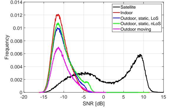
Figure 2: SNR computed on the I-Q samples for each of the considered datasets.
