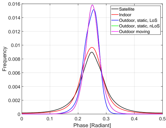
Figure 4: Phase associated with the phasor of the I-Q samples belonging to the first quadrant of the I-Q plane, considering the five different scenarios taken into account in this work.
