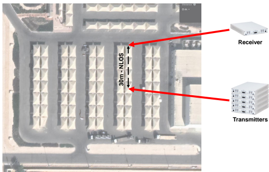
Figure 9: Outdoor scenario with NLoS: we placed the receiver 30 m away from five transmitters in a crowded parking lot.
