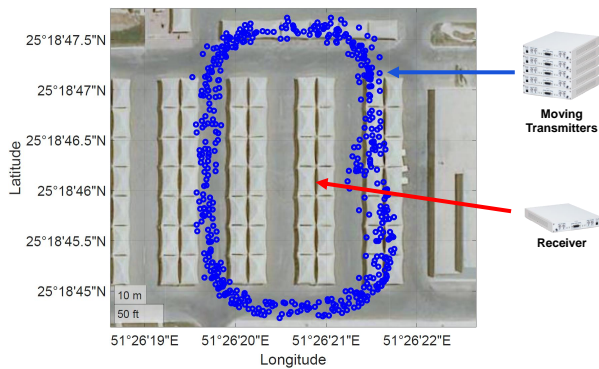
Figure 11: Outdoor Moving Scenario. We considered five different moving transmitters and a static receiver in a crowded parking lot, with the trajectory represented by the blue dots.
