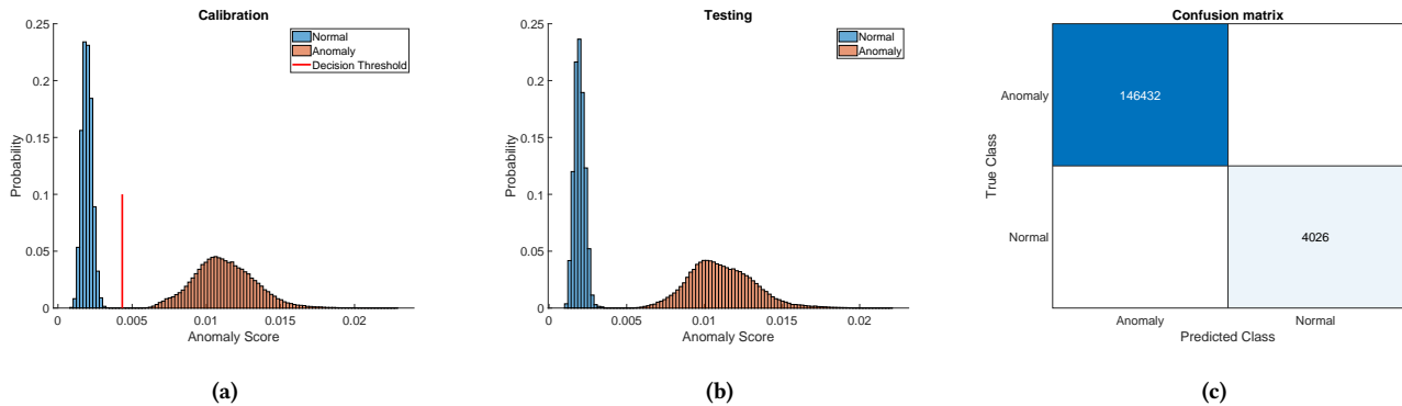
Figure 10: Outdoor scenario, static receiver with nLoS: (a) decision threshold estimation, (b) testing, and (c) confusion matrix.
