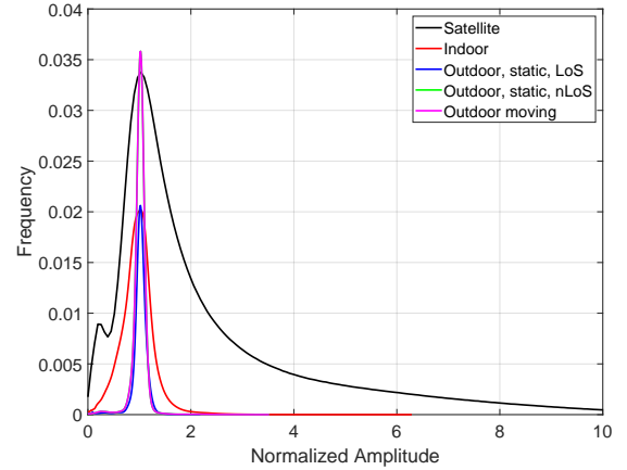
Figure 3: Normalized amplitude of the I-Q samples belonging to the first quadrant of the I-Q plane, considering the five different scenarios taken into account in this work.
