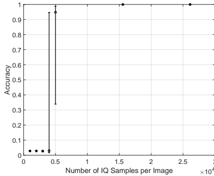
Figure 13: Accuracy as a function of the number of I-Q samples per image, for the static outdoor scenario with nLoS.
