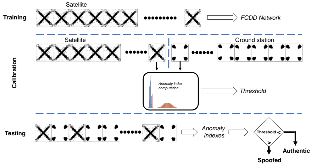
Figure 5: SatPrint in brief: we considered three steps, i.e., (i) training with images generated from satellite I-Q samples, (ii) computation of the threshold from the anomaly indexes, so as to minimize False Positives (FP) and False Negatives (FN), and, (iii) testing sequences of images of both the satellite and ground station, by comparing their anomaly indexes to the threshold.
