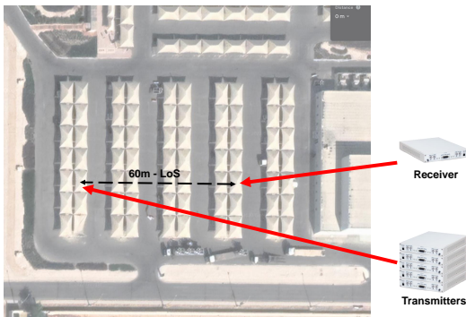
Figure 7: Outdoor scenario with LoS: we considered a parking lot with LoS between the transmitters and the receiver.
